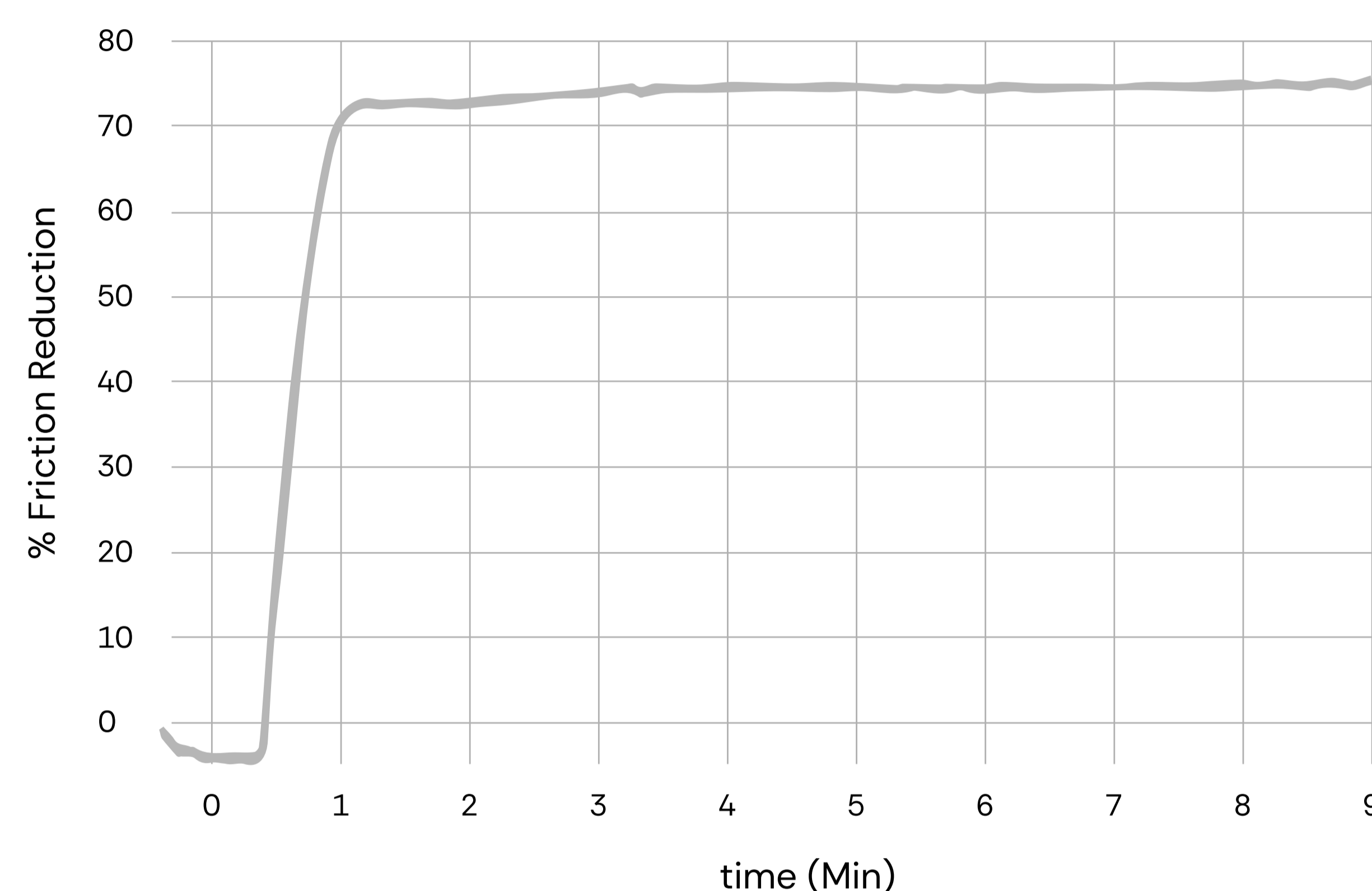
Friction reduction results for Alpha Friction Reducer™ PS 24D in 132,500 ppm TDS water, including 2,800 ppm of calcium, at 2.0 PPT loading.
